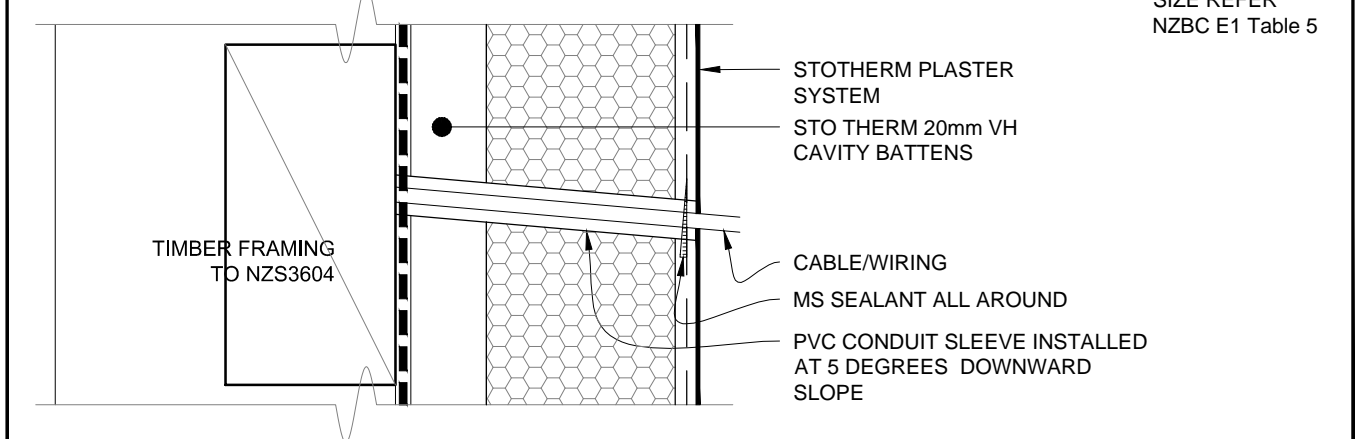
2. WIRING PENETRATION DETAIL
