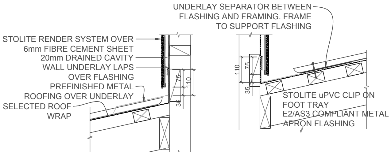
SECTION/FRAMED CHIMNEY SCALE 1:10
