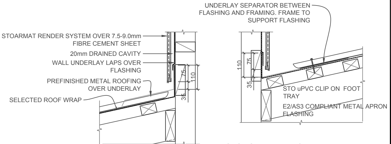
SECTION/FRAMED CHIMNEY SCALE 1:10
