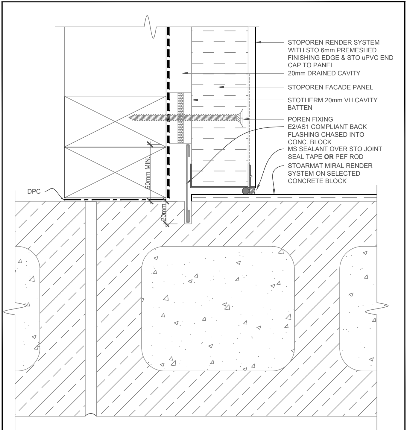
STO S - PROTECT COATING SYSTEM FOR CLEAR FINISHED CONCRETE BLOCK
